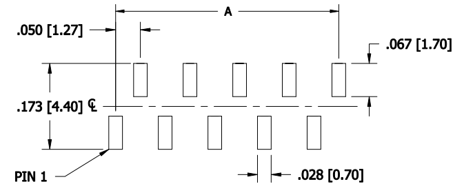
RECOMMENDED P.C.BOARD HOLE LAYOUT LPPB__1NFSD-RC
