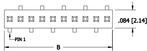
LPPB__1NFSD-RC (OPPOSITE BEND, APPLICABLE ON EVEN PIN COUNTS)
