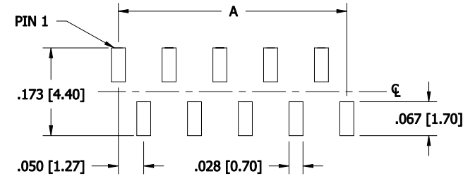
RECOMMENDED P.C.BOARD HOLE LAYOUT LPPB__1NFSC-RC
